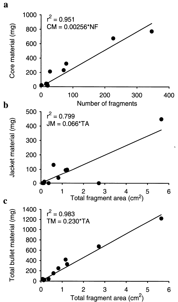
Figure 3. Regression models predicting the mass of (a) core material (CM), (b) jacket material (JM), and (c) total bullet material (TM) in prairie dog carcasses shot with .223 caliber expanding bullets from the number of bullet fragments (NF) and total surface area (TA) of bullet fragments in the radiographs of the carcasses, Thunder Basin, Wyoming, USA, 2004. We used these models to predict the mass of each bullet component for carcasses from which we had not extracted fragments.
